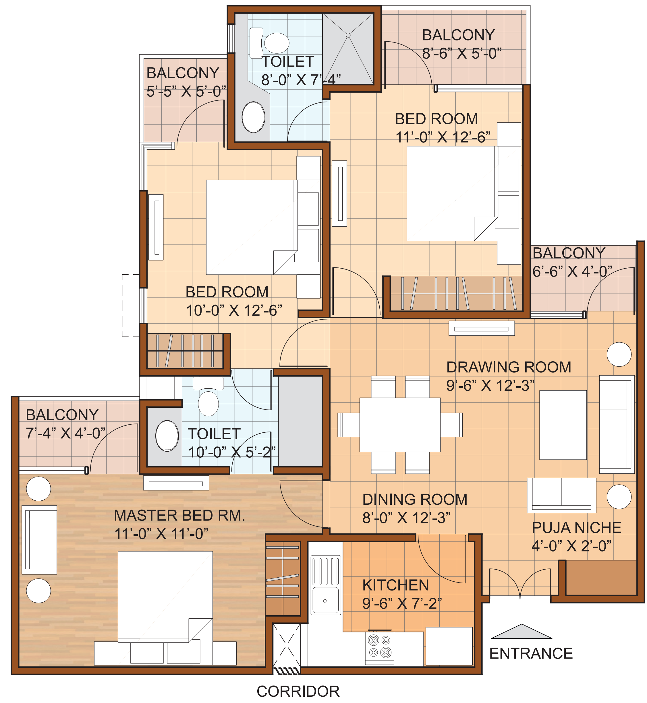
FLOOR PLAN
